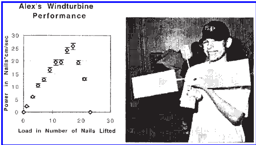
FIGURE 7 Wind turbine challenge. Students test their turbine designs making measurement in an airflow. Their measurements are independent of teacher assessment. Here they measure the time it takes to lift weights over a standard distance and graph their results. Note that the roughly parabolic shape shows features of stall load and free rotation. Bars enclose \pm 1 -sec error in time measurement and \pm 1 cm in distance measurement.
